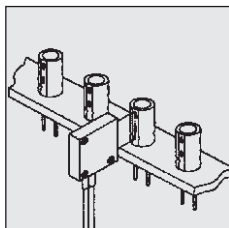
Label detection
